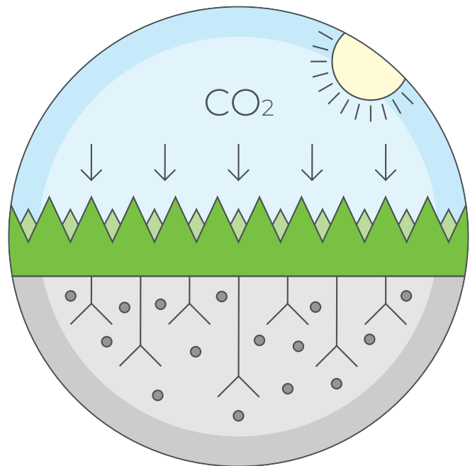
Carbon is absorbed through grass canopy during photosynthesis and sequestered through the fibrous root system into the soil as plants senesce and decompose.
